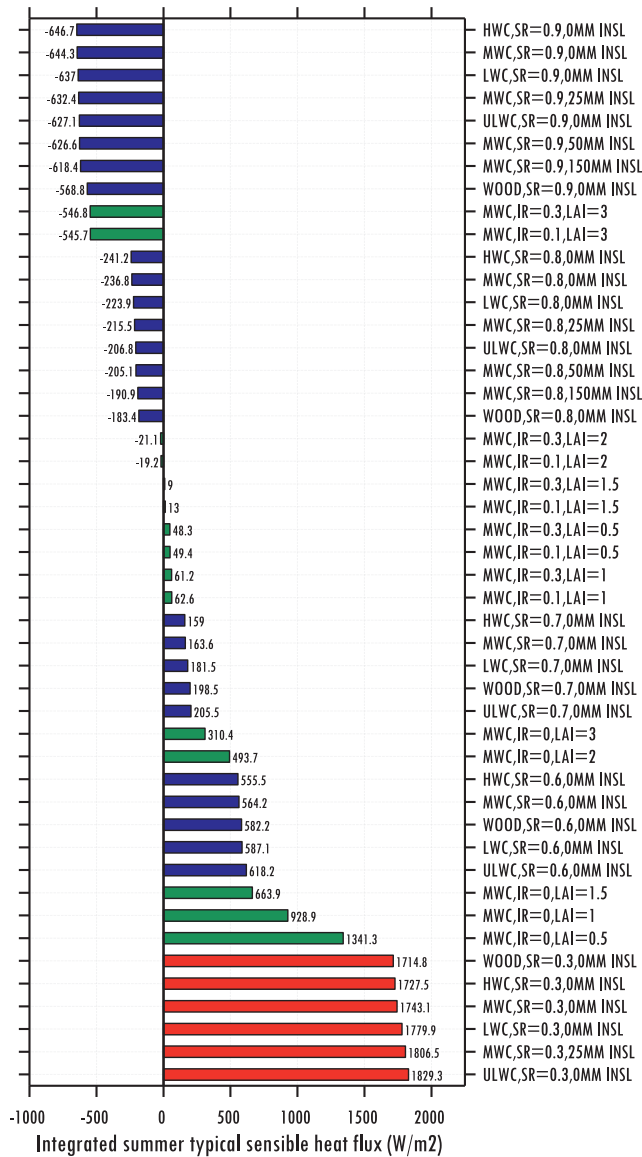
Fig. 13. Integrated sensible heat flux for a typical summer design day extracted for various cool and green roof configurations in Singapore.
