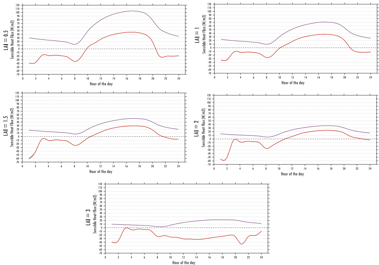
Fig. 12. Comparison of Sensible Heat flux differences between green roofs for various LAI and IR Blue line – Non irrigated green roof (IR-0) Red Line – Irrigated green roof (IR-0.1/0.3). (For interpretation of the references to colour in this figure legend, the reader is referred to the web version of this article.)
