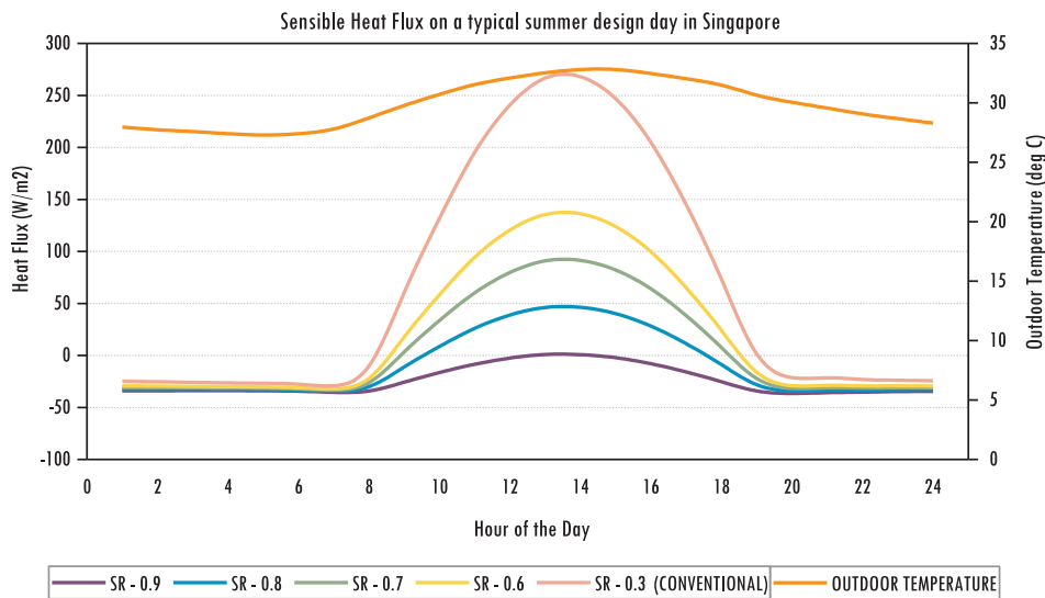
Fig. 3. Sensible Heat flux for a typical construction on a typical summer design day in Singapore with various solar reflectance scenarios.
