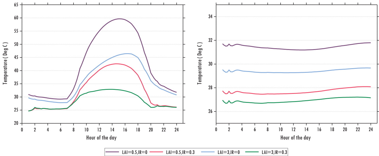
Fig. 11. Comparison of Inside temperature differences between conventional roof and non irrigated green roofs for various LAI.
