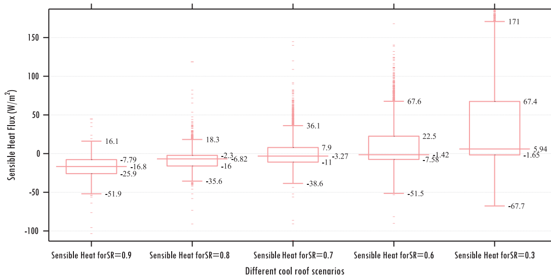
Fig. 2. Comparison of UHI mitigation potential for a typical construction between different cool roof albedos and conventional roof.
