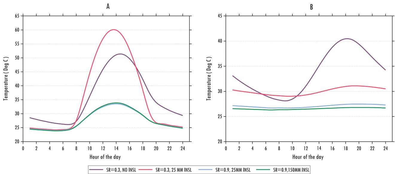
Fig. 9. (A). Surface outside temperature for different roofs with various insulation levels for a typical summer design day. (B). Surface inside temperature for different roofs with various insulation levels for a typical summer design day.
