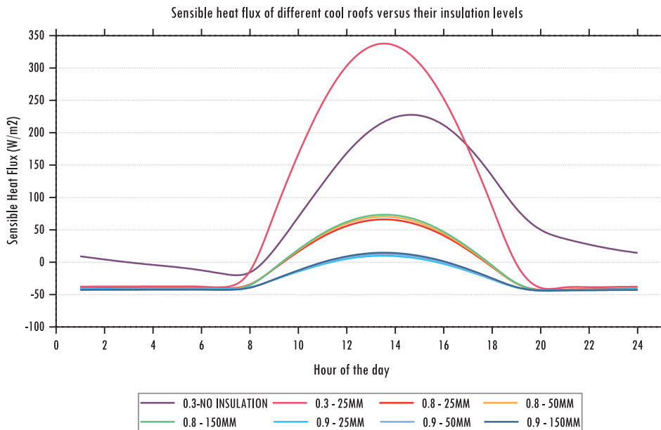
Fig. 8. Sensible Heat flux released from different cool roof scenarios with various insulation levels for a typical summer design day.
