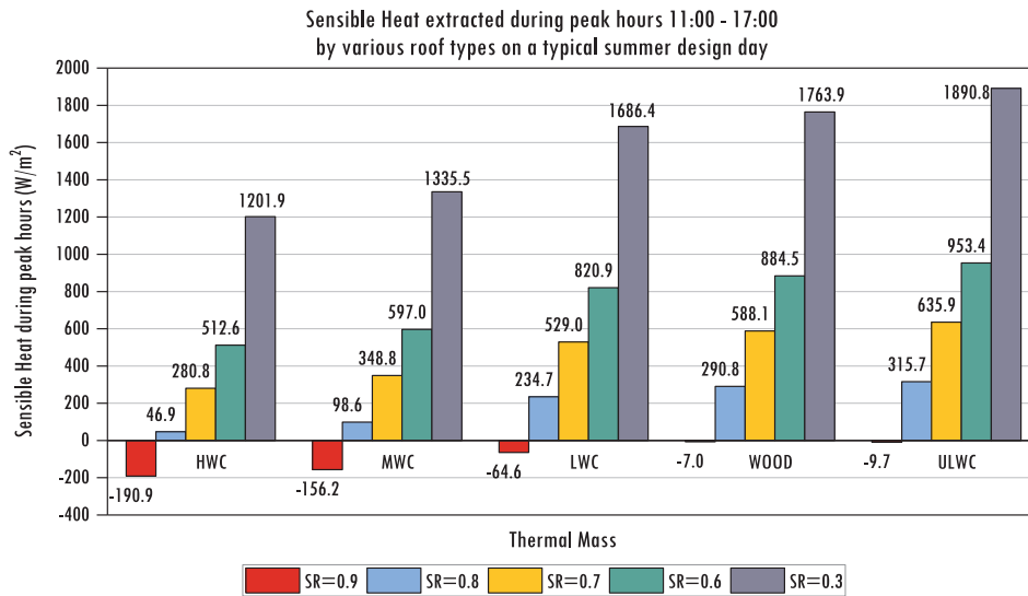
Fig. 7. Integrated sensible Heat for various thermal mass levels of the roof during a typical summer design day for Singapore.
