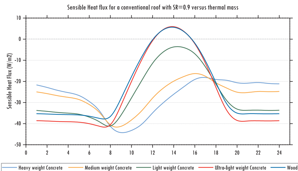
Fig. 5. Sensible Heat flux versus thermal mass for a cool roof with SR = 0.9 for Singapore.
