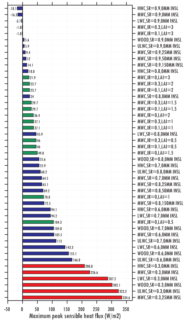
Fig. 14. Maximum sensible heat flux released for a typical summer design day for various cool and green roof configurations in Singapore.
