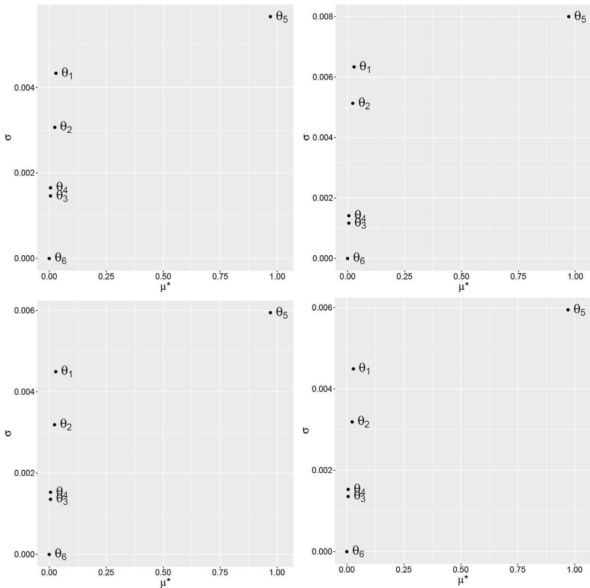
Fig. 1. Scatter plots of the Morris sensitivity measures for various parameters of different zones.
