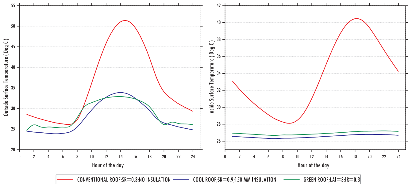
Fig. 16. Outside and Inside surface temperature comparisons for conventional roof, best cool roof and best green roof scenarios.
