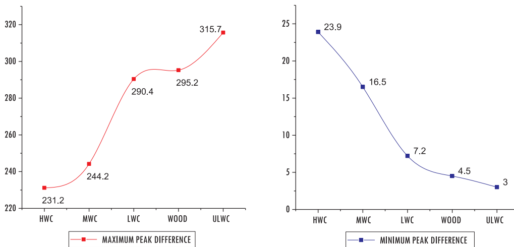
Fig. 6. Comparison between maximum and minimum peak differences for various thermal mass configurations.
