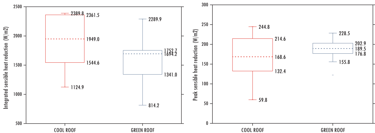
Fig. 15. Integrated and peak sensible heat reduction for a typical summer design day for various cool and green roof configurations in Singapore.
