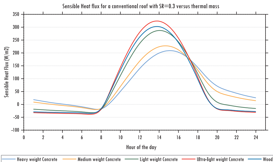
Fig. 4. Sensible Heat flux versus thermal mass for a cool roof with SR = 0.3 for Singapore.
