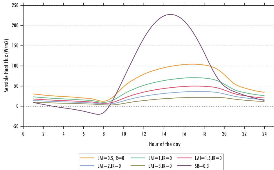
Fig. 10. Sensible heat flux released from green roofs with no irrigation rate for a typical summer design day.
